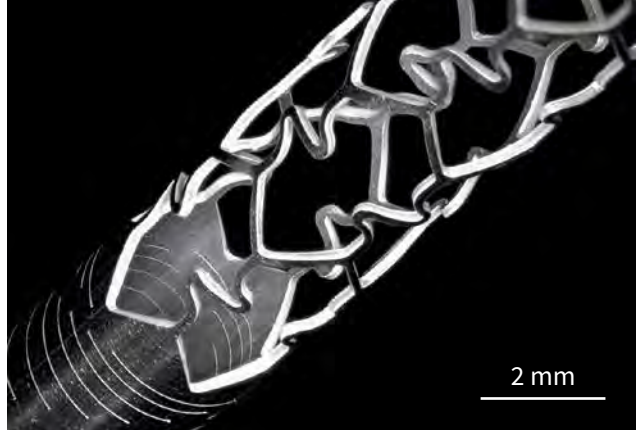
Stent cut using CARBIDE laser. Source: Amada Miyachi America.
