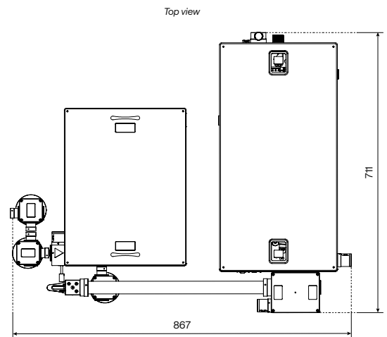
ORPHEUS-PS with SHBC drawing
