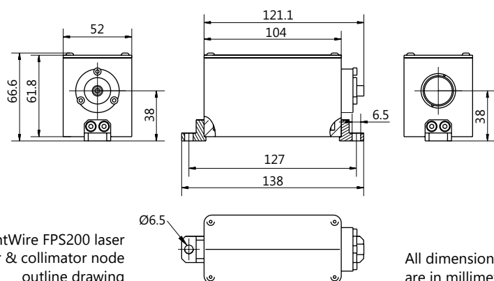
LighWire FPS series "Compact" version drawing. Example only. Actual dimensions depends on a selected laser configuration and options. Please enquire
