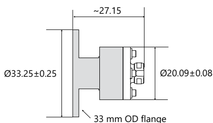
LightWire FPS10/100 laser collimator flange outline drawing for beam diameters 0.9 mm and 1.3 mm
