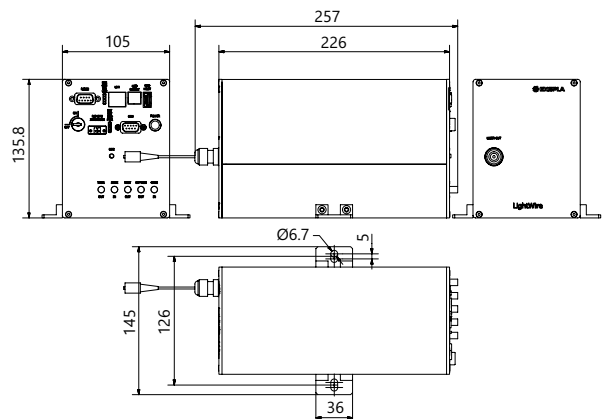
LighWire FPS series "Compact" version drawing. Example only. Actual dimensions depends on a selected laser configuration and options. Please enquire
