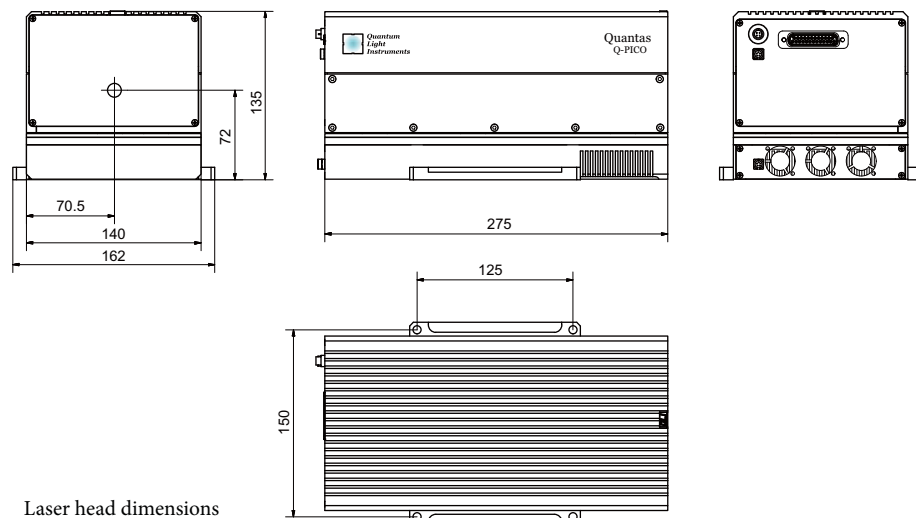
Laser head dimensions
