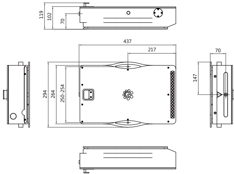
Outline drawing of FemtoLux 3 laser head
