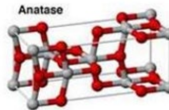
Crystal Structures of \text{TiO}_2 nanoparticles
