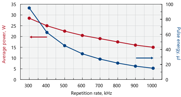
Typical output power and energy curves of Atlantic GR25
