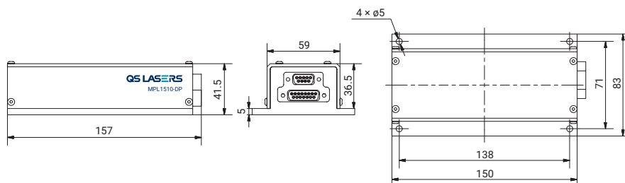
Laser head dimensions
