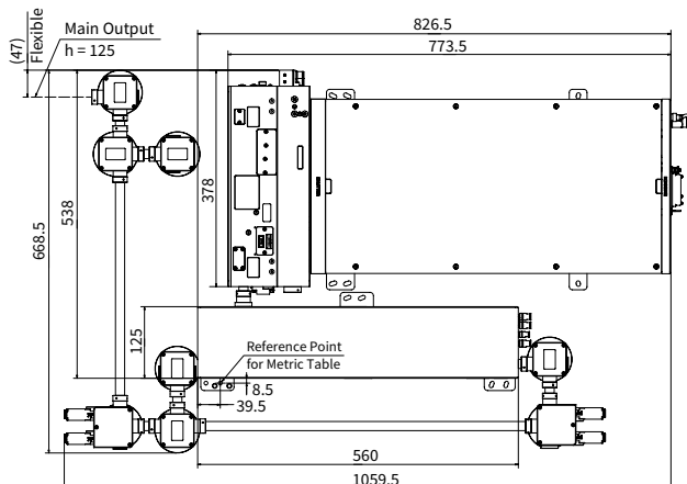
CRONUS-3P with optional beam steering drawing
