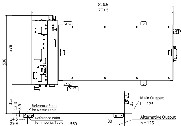
CRONUS-3P drawing
