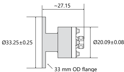
LightWire FFS100CHI/200 laser collimator flange outline drawing for beam diameter 2.1/2.0 mm
