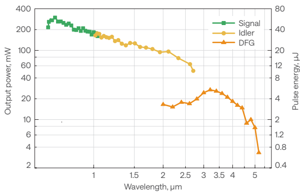
ORPHEUS-PS tuning curves Pump: 5 W, 1000 μJ, 5 kHz from PHAROS-20W-SP
